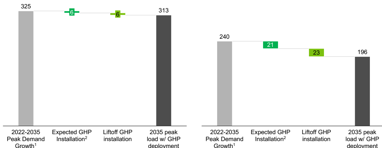
Figure 32: Reduction potential of Summer (left) and Winter (right) peak demand (GW) between 2022 and 2035 under a highly-electrified future scenario.
