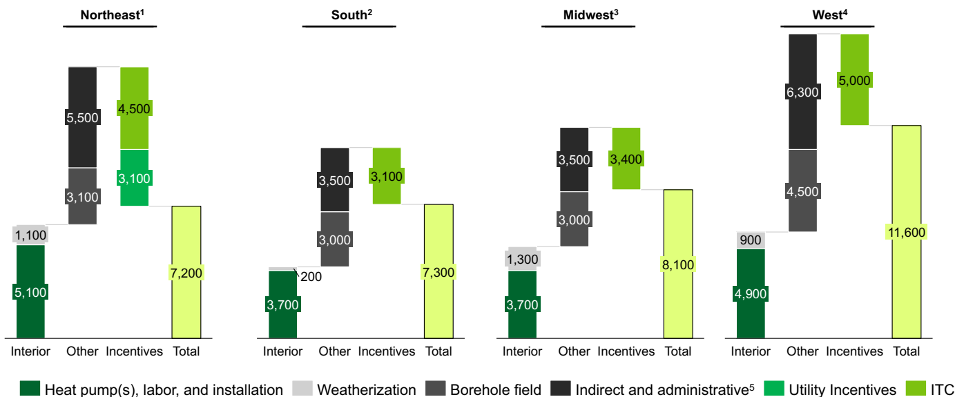
Figure 20: Regional cost estimates for residential geothermal heat pump retrofits.
