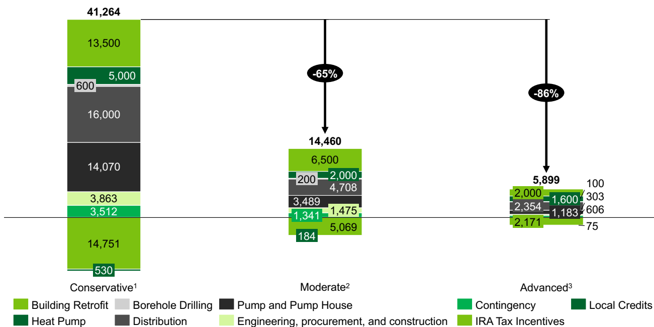
Figure 21: Estimated costs of community-scale TENS
