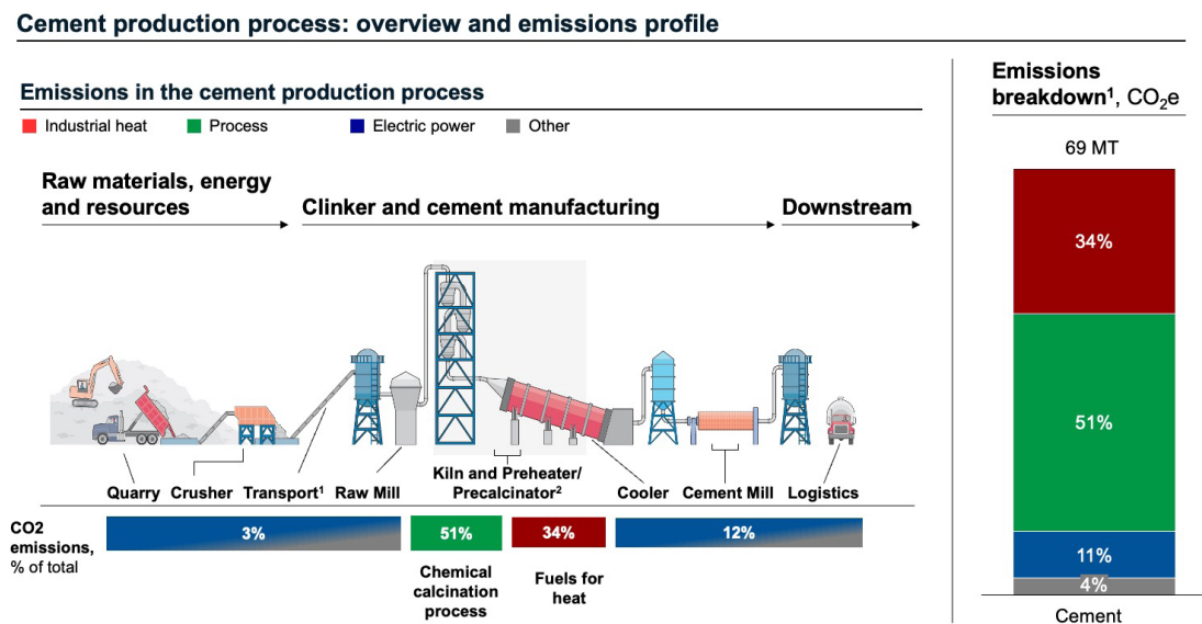
Figure 2.1. Overview of the cement production process with corresponding emissions by source. 85% of emissions come from clinker production in the preheater/precalciner and kiln, of which 51% are intrinsic to the chemical calcination process and 34% come from the combustion of fuels for heat.
