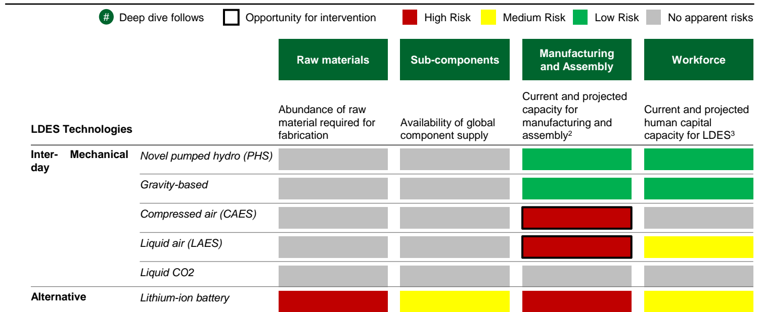
Figure 14: Inter-day LDES systems have fewer supply chain vulnerabilities compared to Li-ion alternatives. xxxii 1 Excludes geographies with potential access issues as assessed by DOE. U.S. and global supply chains were assessed separately but combined on this page; 3 For example, available supply of components, operational manufacturing capacity; 5 Highly-skilled and specialized talent for design and technical components and systems, highly skilled (likely unionized) talent for construction and operations
